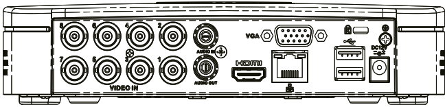
Rear Panel
