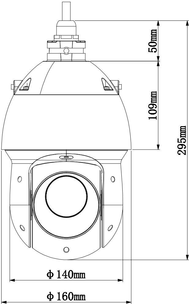
Dimensions (mm/inch)
